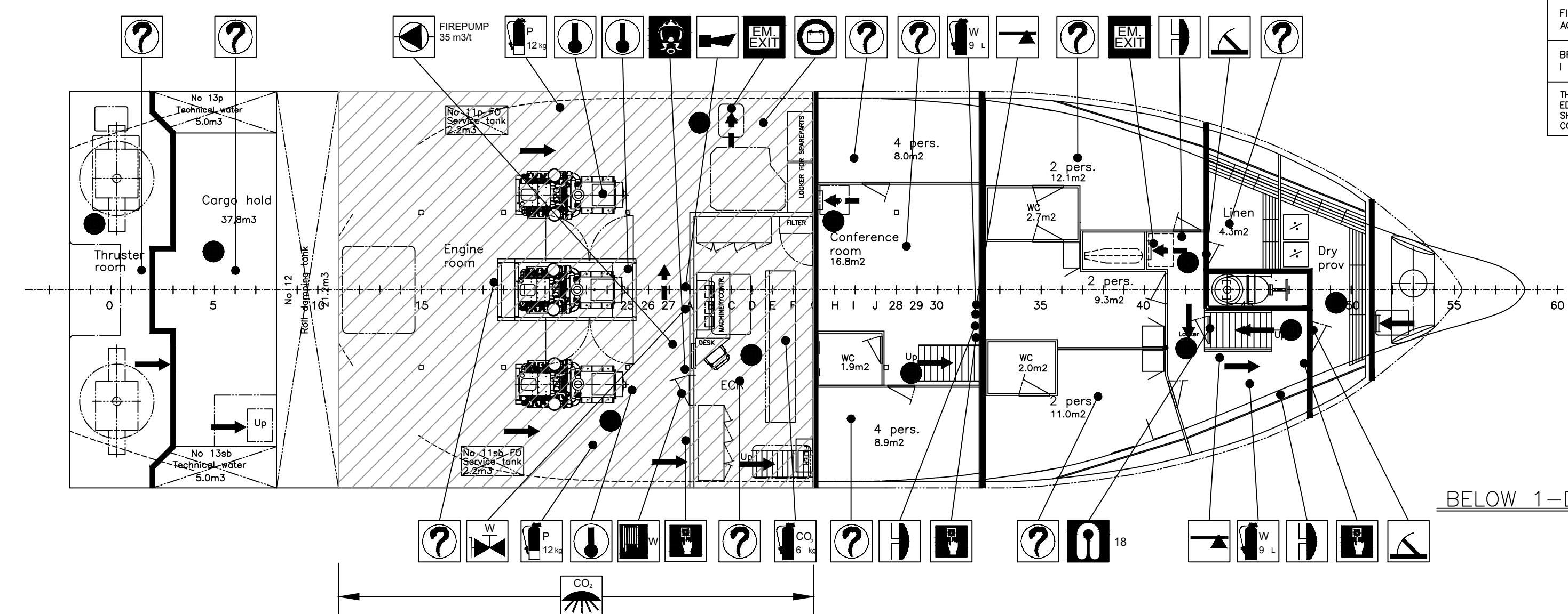
1-DECK
