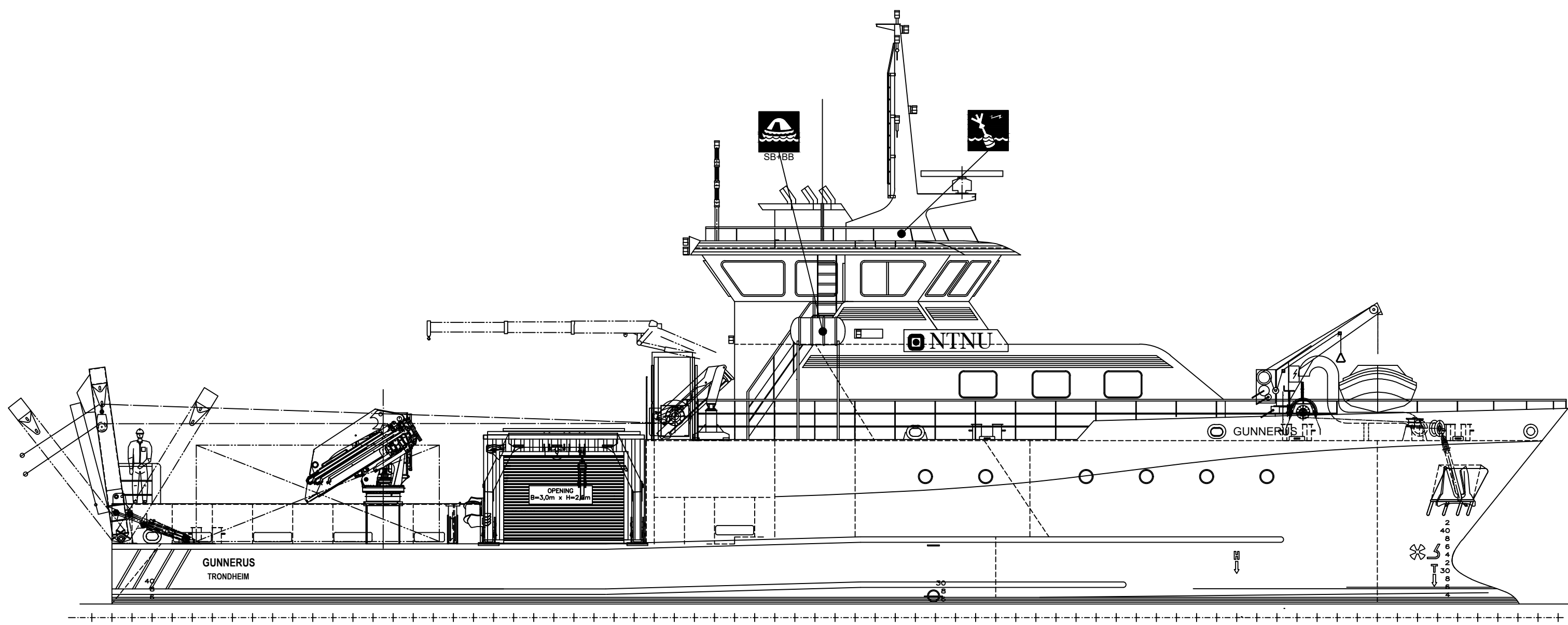
PROFILE
